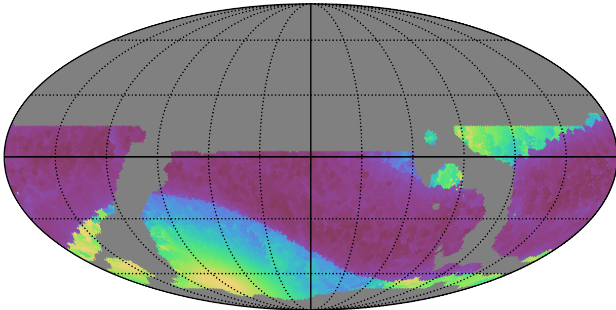
weather_cloudso20v3.4_10yrs WFD all bands: Min solarElong
