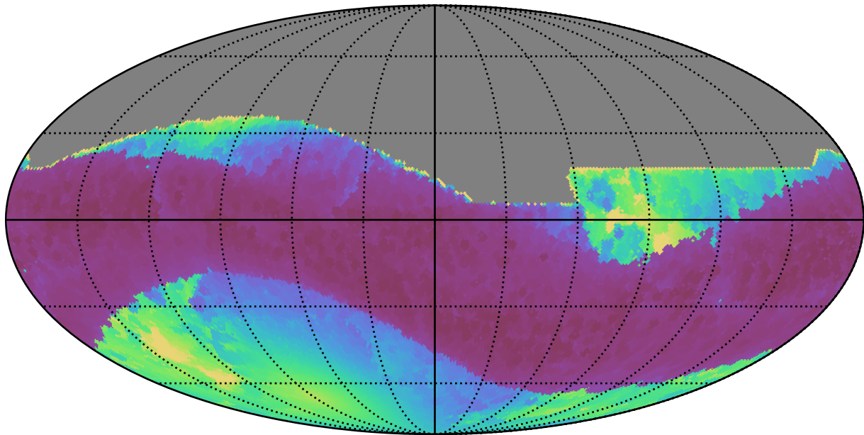
weather_cloudso20v3.4_10yrs All sky all bands: Min solarElong
