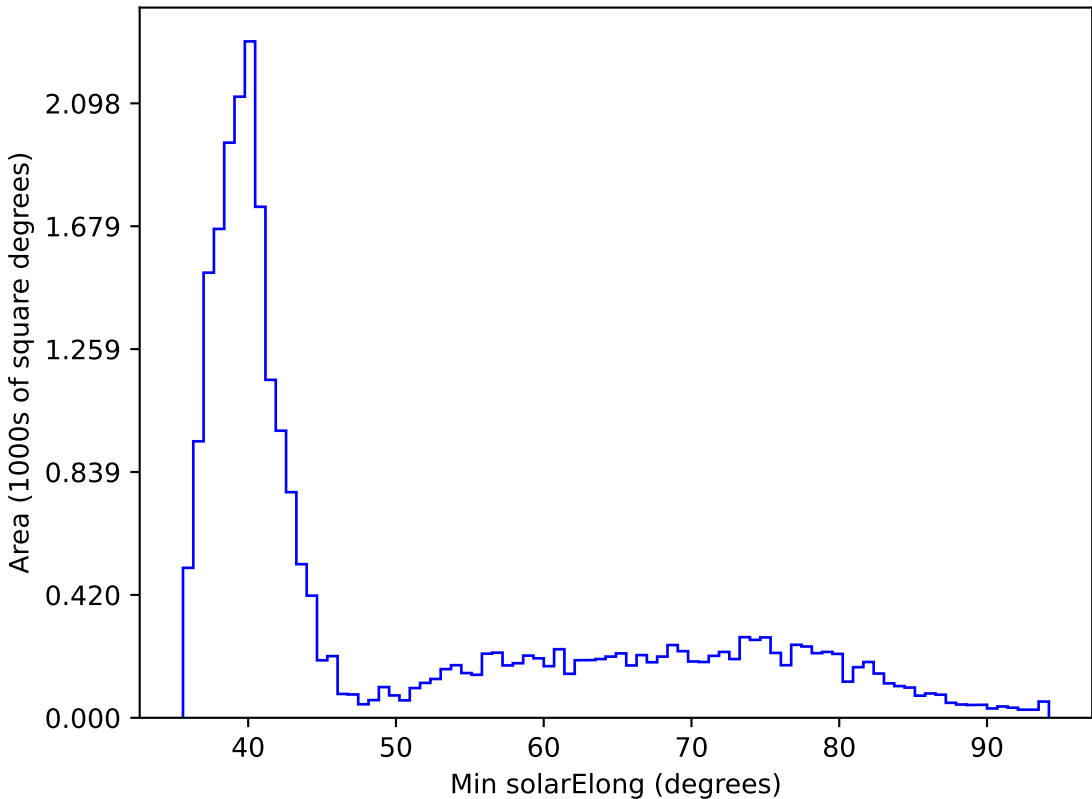
weather_cloudso20v3.4_10yrs All sky all bands: Min solarElong
