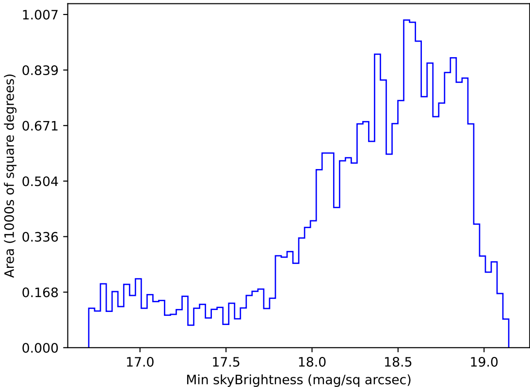
weather_cloudso20v3.4_10yrs Yr 1 z band: Min skyBrightness
