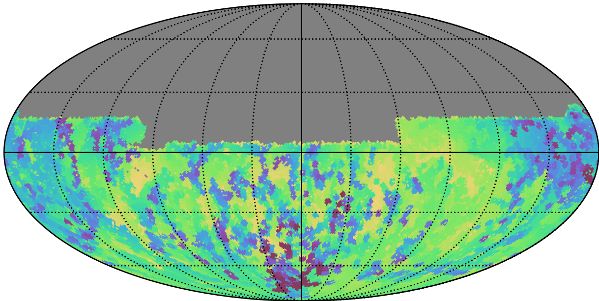
weather_cloudso20v3.4_10yrs Yr 1 y band: Min skyBrightness
