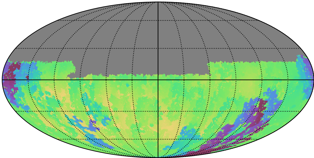
weather_cloudso20v3.4_10yrs Yr 1 u band: Min skyBrightness
