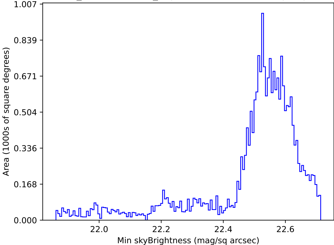
weather_cloudso20v3.4_10yrs Yr 1 u band: Min skyBrightness
