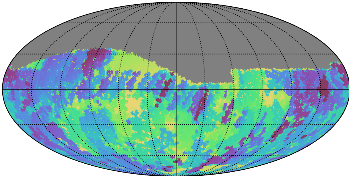
weather_cloudso20v3.4_10yrs Yr 1 r band: Min skyBrightness
