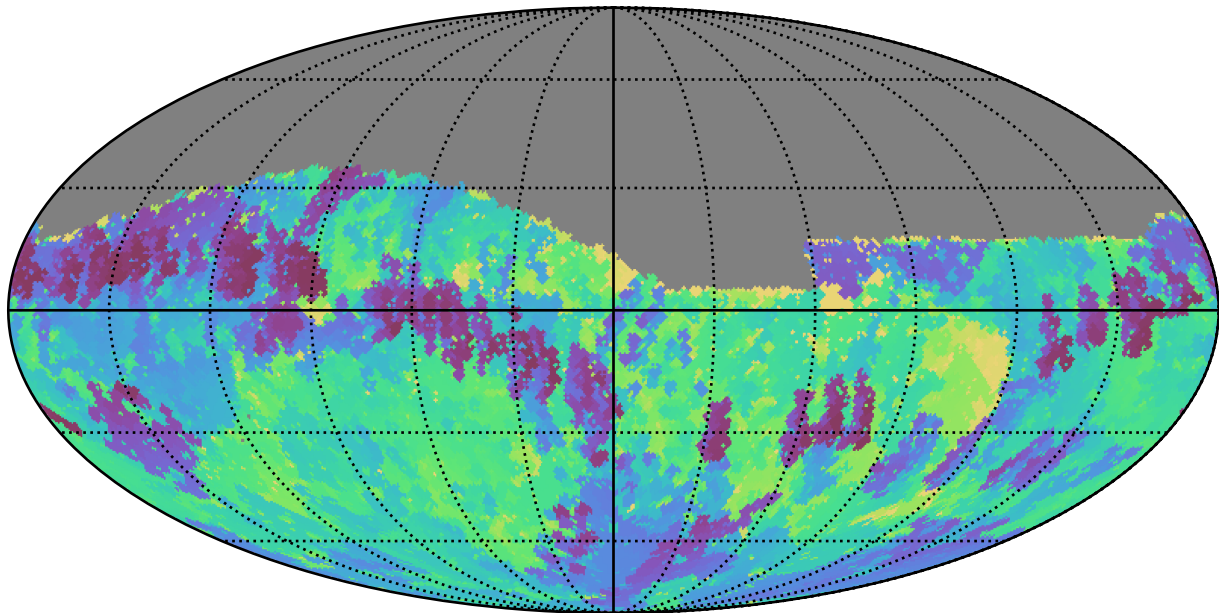
weather_cloudso20v3.4_10yrs Yr 1 i band: Min skyBrightness
