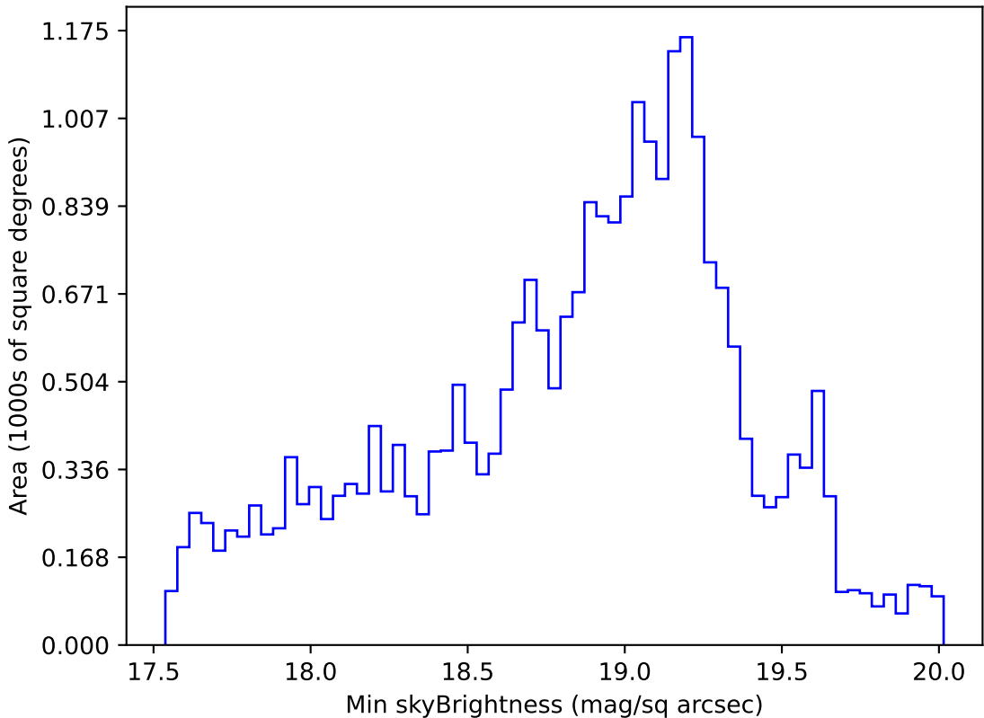
weather_cloudso20v3.4_10yrs Yr 1 i band: Min skyBrightness
