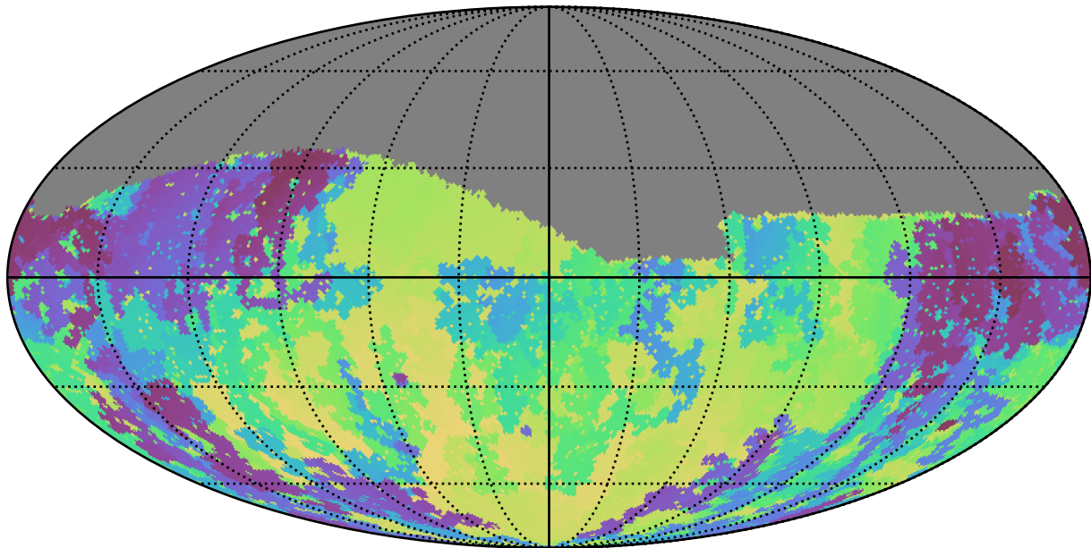
weather_cloudso20v3.4_10yrs Yr 1 g band: Min skyBrightness
