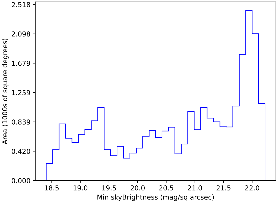
weather_cloudso20v3.4_10yrs Yr 1 g band: Min skyBrightness
