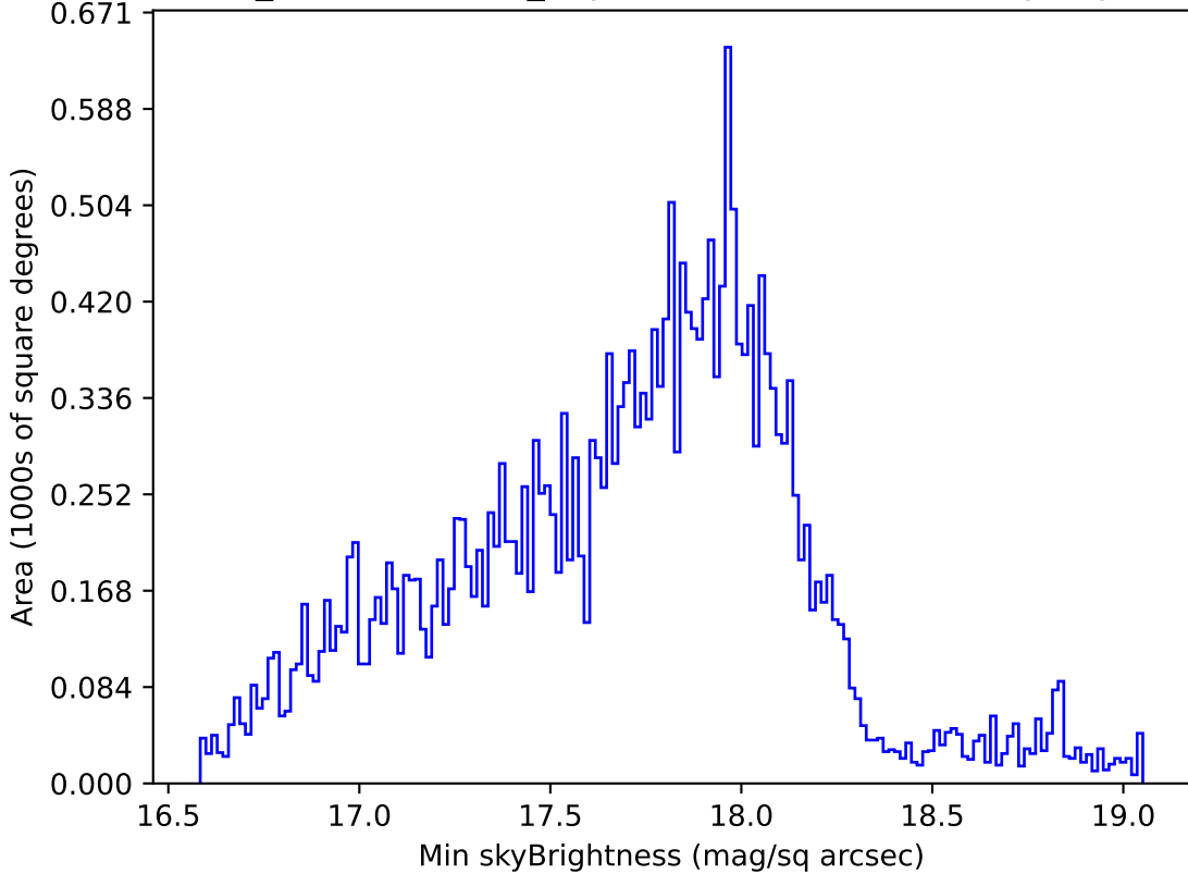
weather_cloudso20v3.4_10yrs Yr 1 all bands: Min skyBrightness
