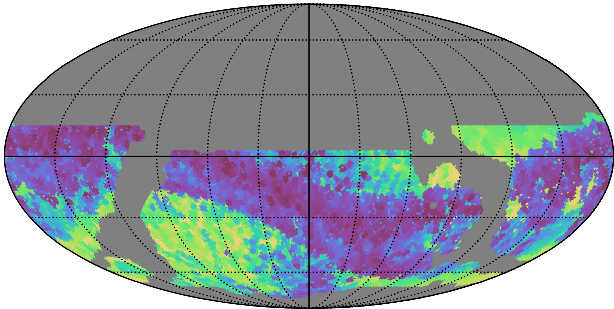
weather_cloudso20v3.4_10yrs WFD z band: Min skyBrightness
