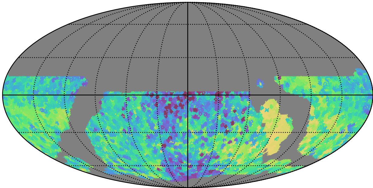
weather_cloudso20v3.4_10yrs WFD y band: Min skyBrightness
