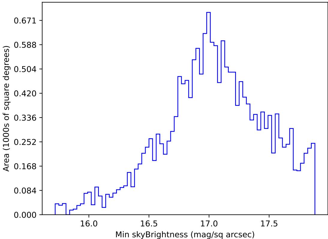
weather_cloudso20v3.4_10yrs WFD y band: Min skyBrightness
