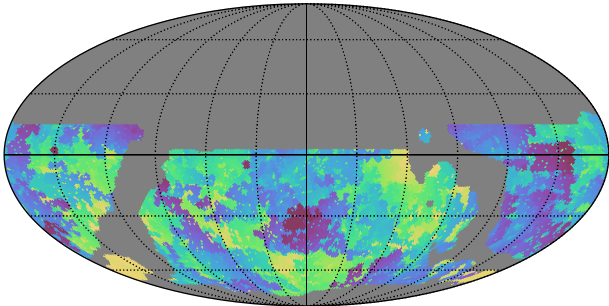
weather_cloudso20v3.4_10yrs WFD u band: Min skyBrightness
