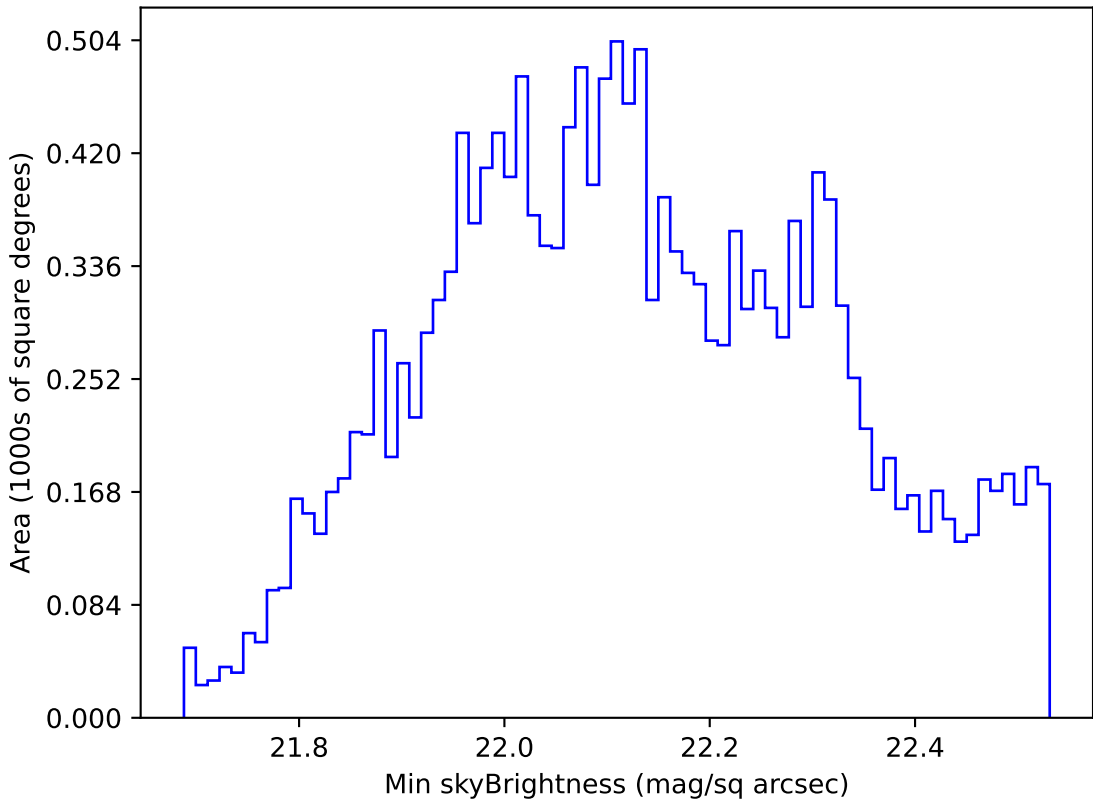
weather_cloudso20v3.4_10yrs WFD u band: Min skyBrightness
