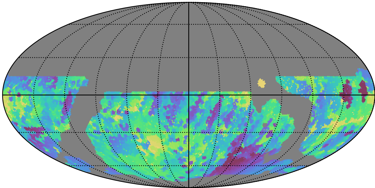
weather_cloudso20v3.4_10yrs WFD r band: Min skyBrightness
