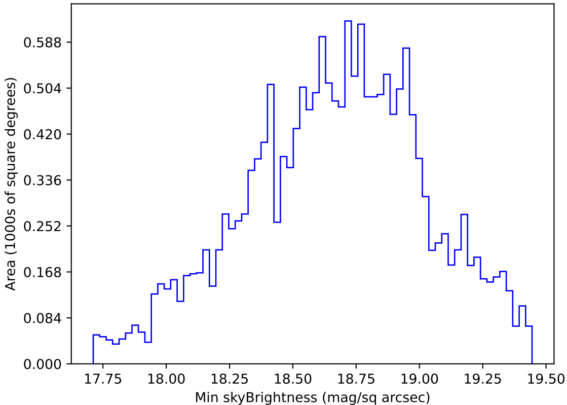
weather_cloudso20v3.4_10yrs WFD r band: Min skyBrightness
