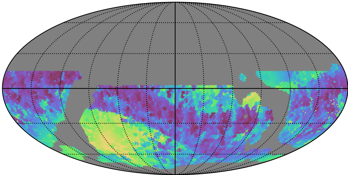
weather_cloudso20v3.4_10yrs WFD i band: Min skyBrightness
