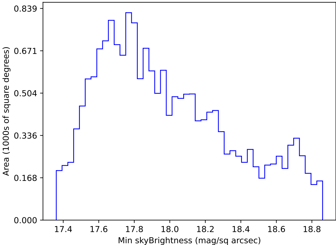
weather_cloudso20v3.4_10yrs WFD i band: Min skyBrightness
