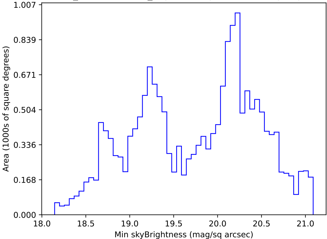
weather_cloudso20v3.4_10yrs WFD g band: Min skyBrightness
