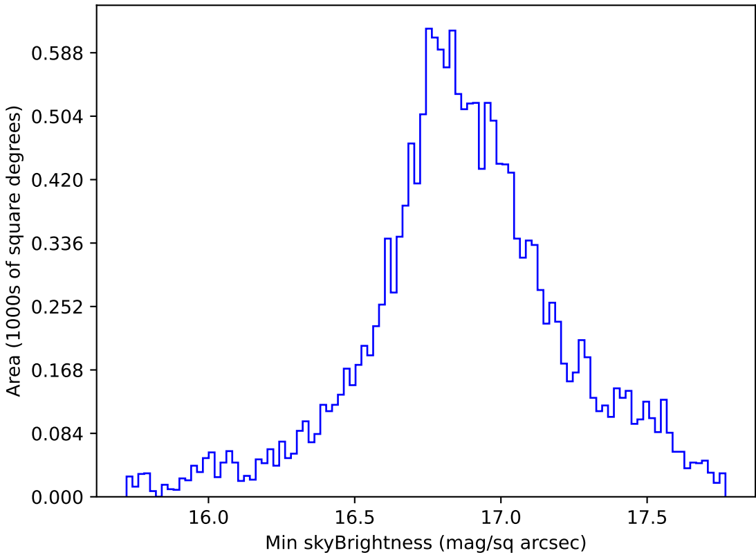
weather_cloudso20v3.4_10yrs WFD all bands: Min skyBrightness
