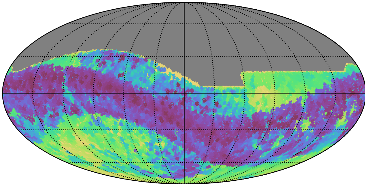
weather_cloudso20v3.4_10yrs All sky z band: Min skyBrightness
