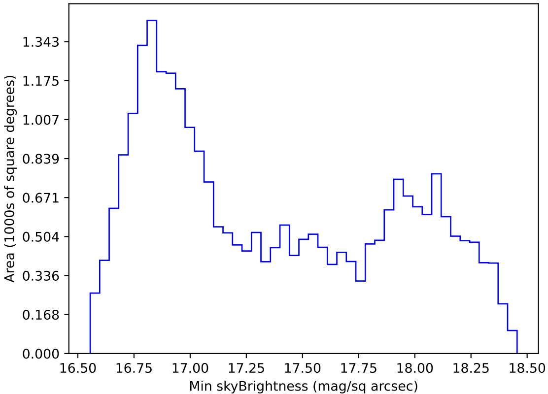
weather_cloudso20v3.4_10yrs All sky z band: Min skyBrightness
