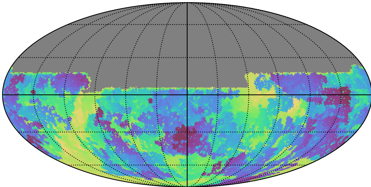
weather_cloudso20v3.4_10yrs All sky u band: Min skyBrightness
