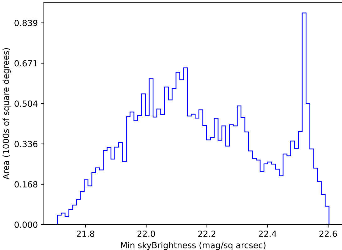
weather_cloudso20v3.4_10yrs All sky u band: Min skyBrightness
