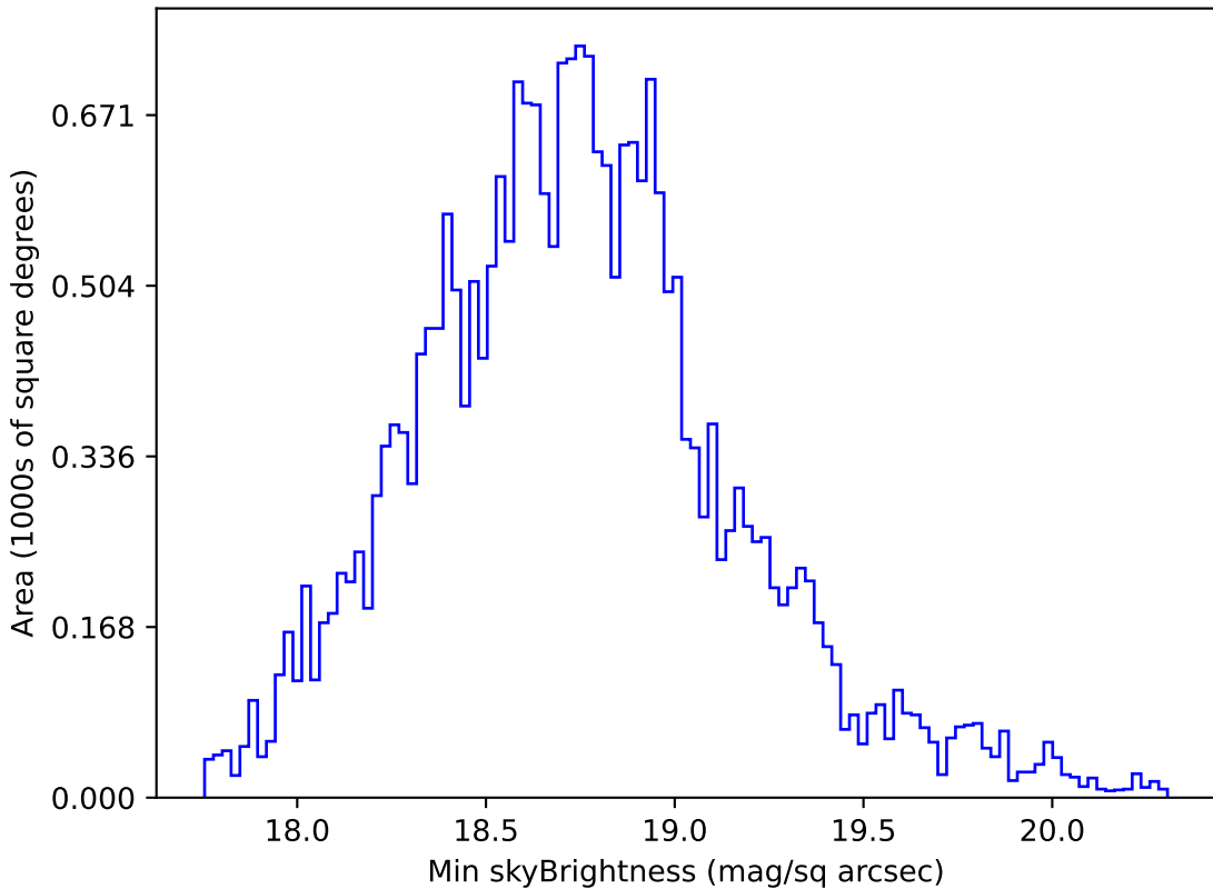
weather_cloudso20v3.4_10yrs All sky r band: Min skyBrightness
