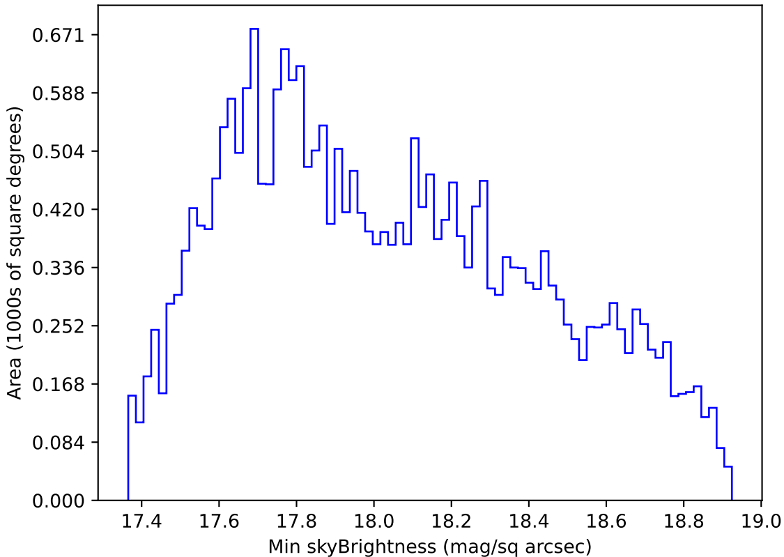
weather_cloudso20v3.4_10yrs All sky i band: Min skyBrightness
