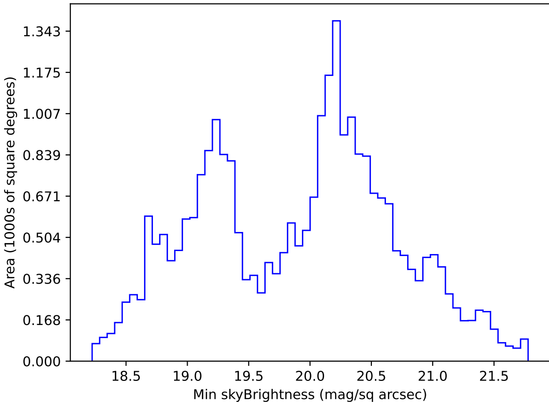
weather_cloudso20v3.4_10yrs All sky g band: Min skyBrightness
