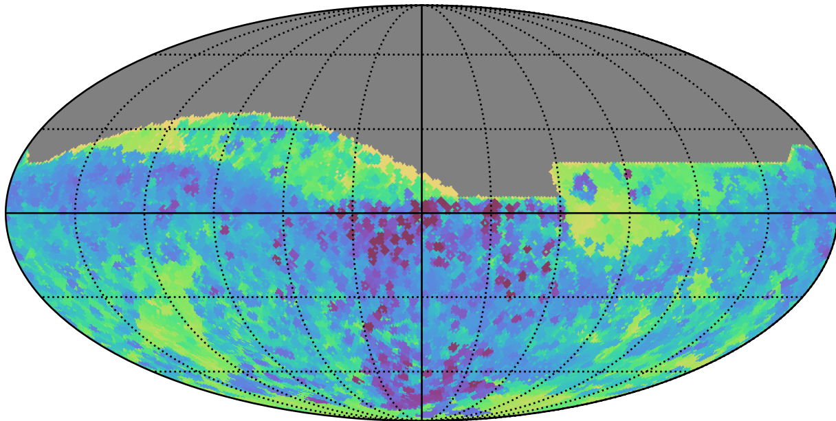
weather_cloudso20v3.4_10yrs All sky all bands: Min skyBrightness
