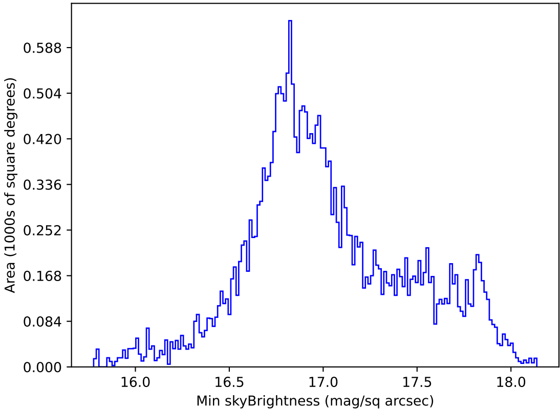
weather_cloudso20v3.4_10yrs All sky all bands: Min skyBrightness
