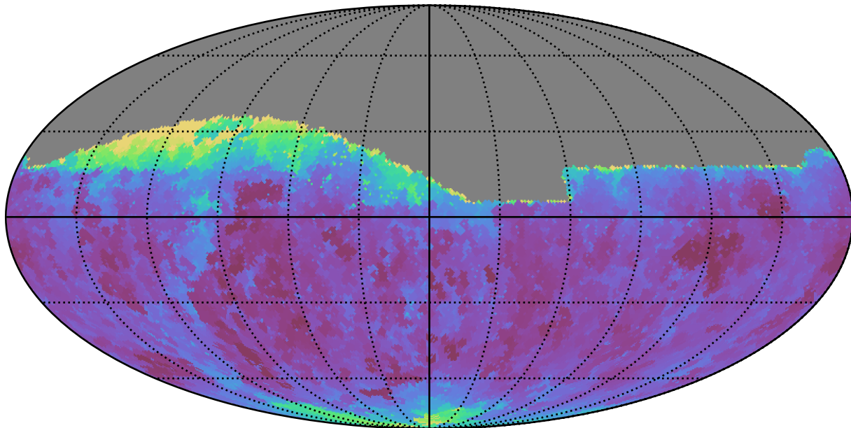
weather_cloudso20v3.4_10yrs Yr 1 all bands: Min seeingGeom
