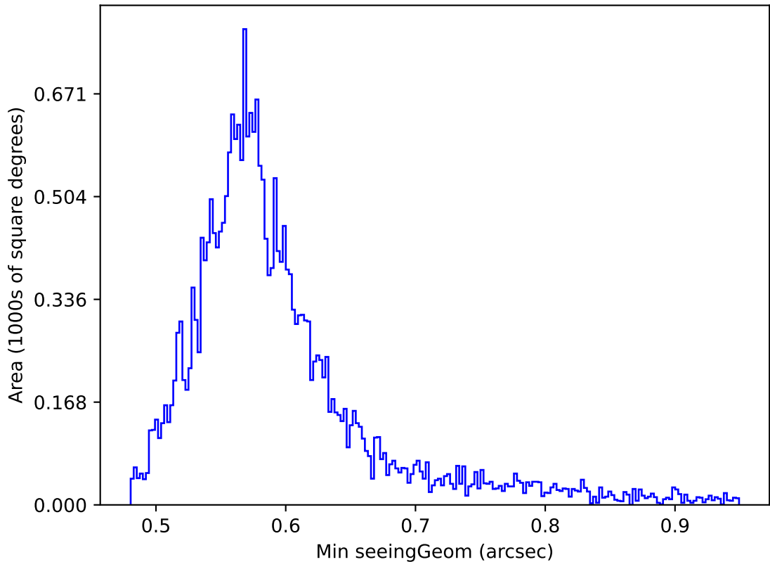
weather_cloudso20v3.4_10yrs Yr 1 all bands: Min seeingGeom
