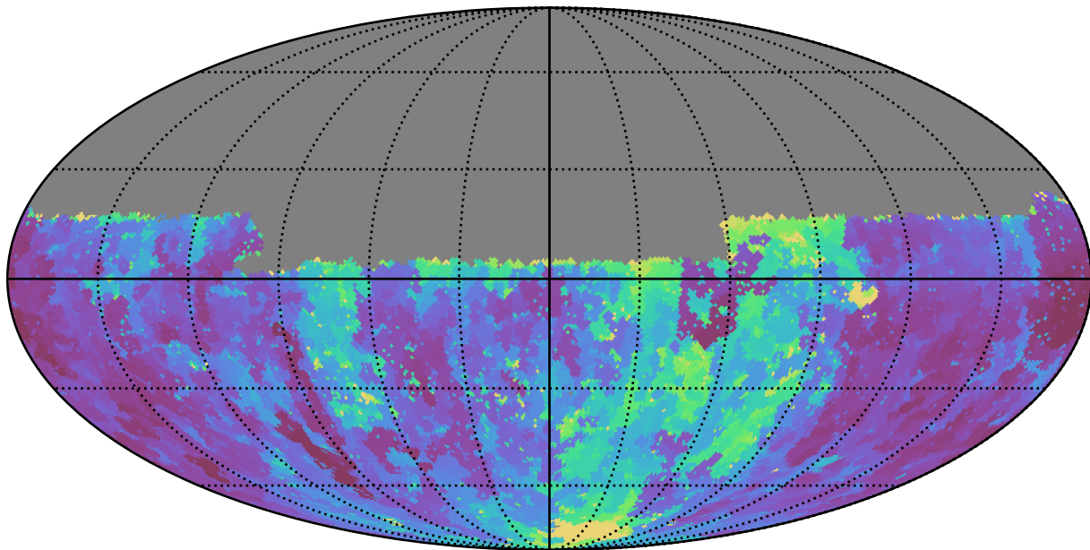
weather_cloudso20v3.4_10yrs Yr 1 u band: Min seeingEff
