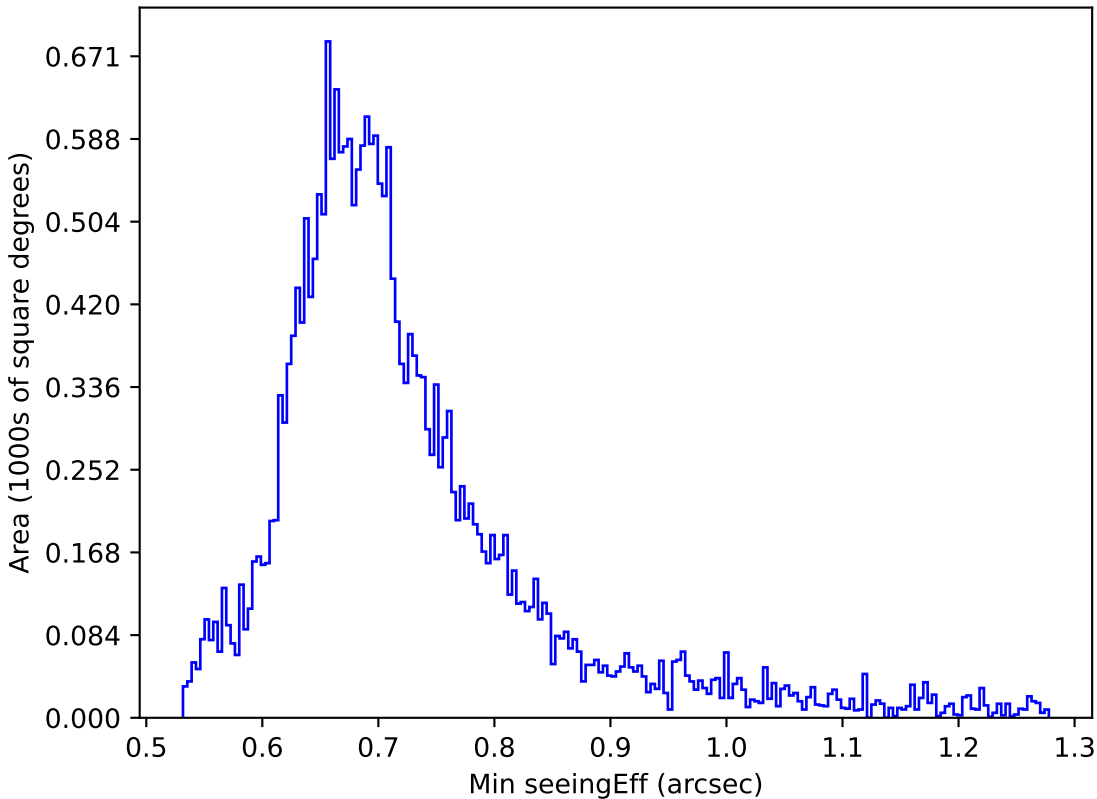
weather_cloudso20v3.4_10yrs Yr 1 r band: Min seeingEff
