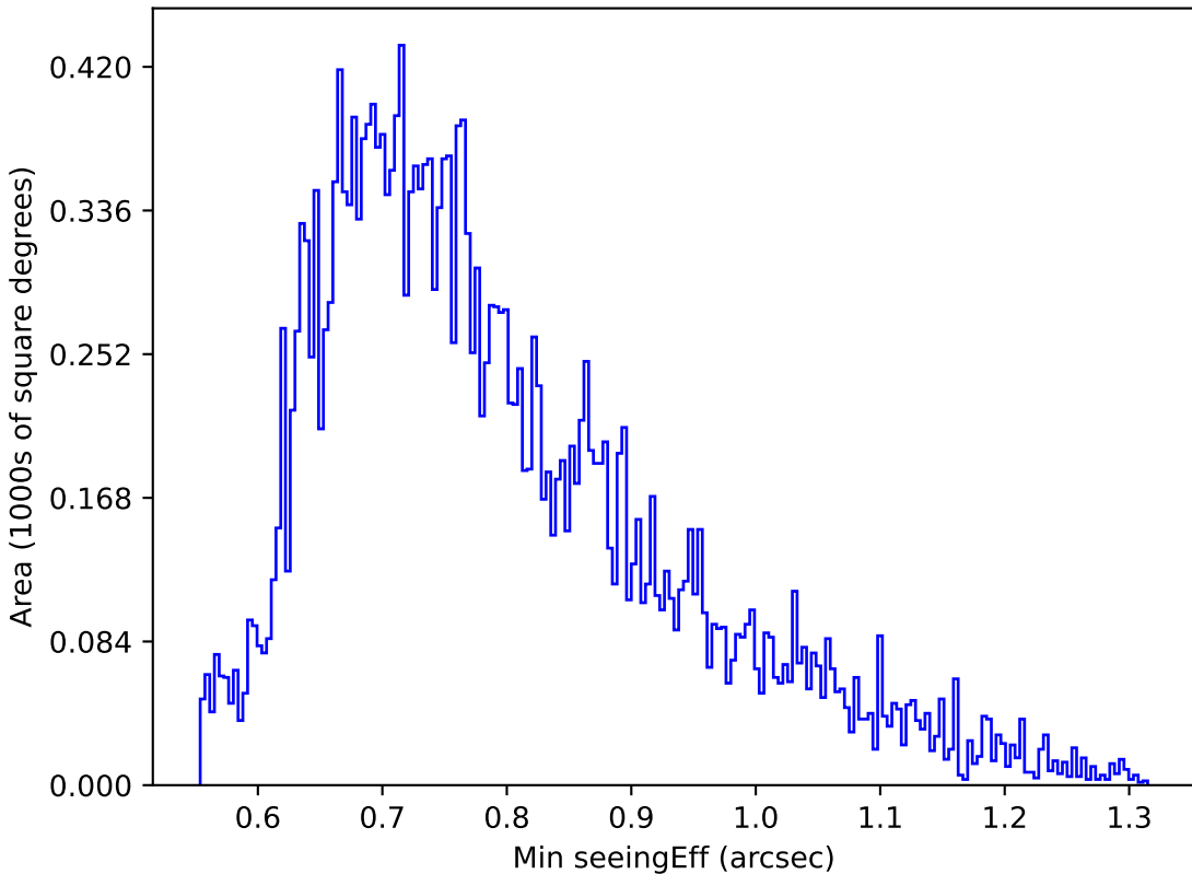
weather_cloudso20v3.4_10yrs Yr 1 g band: Min seeingEff
