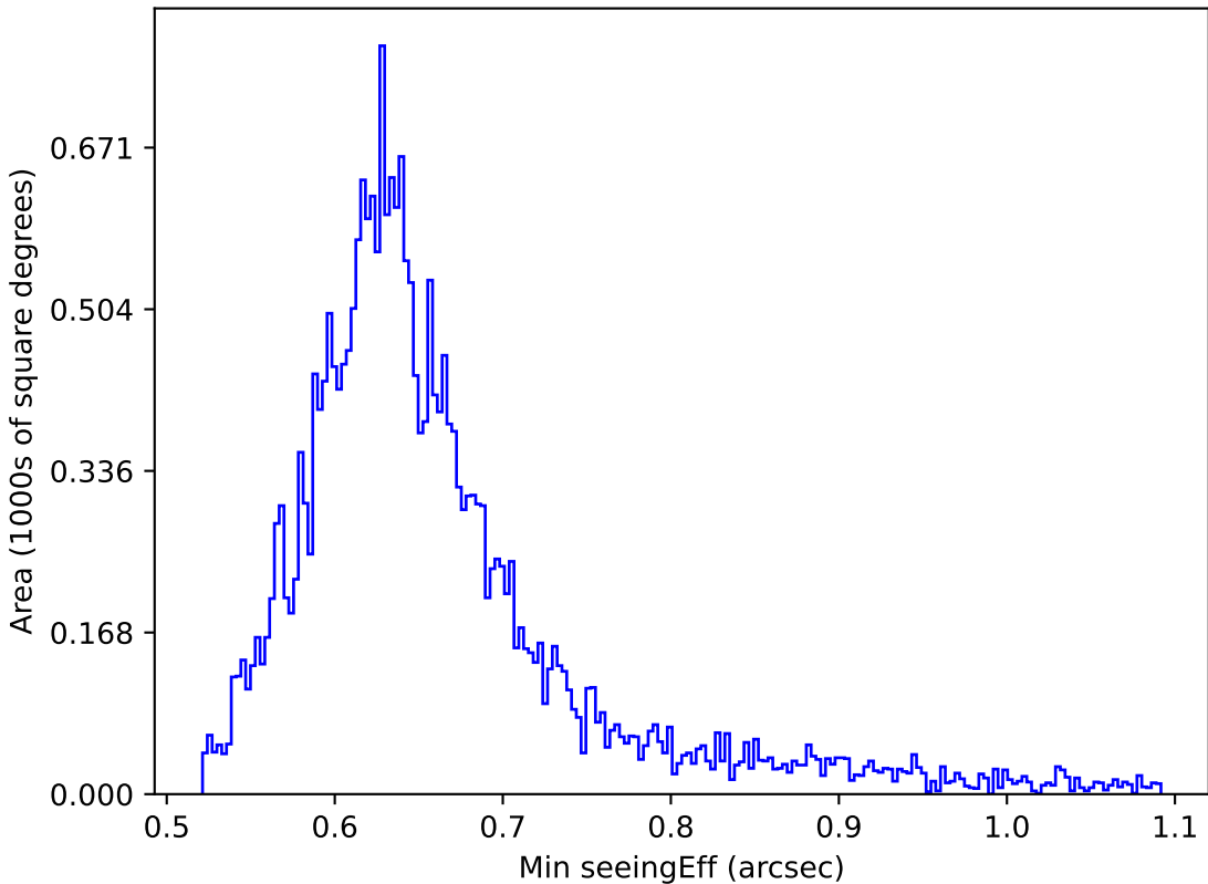
weather_cloudso20v3.4_10yrs Yr 1 all bands: Min seeingEff
