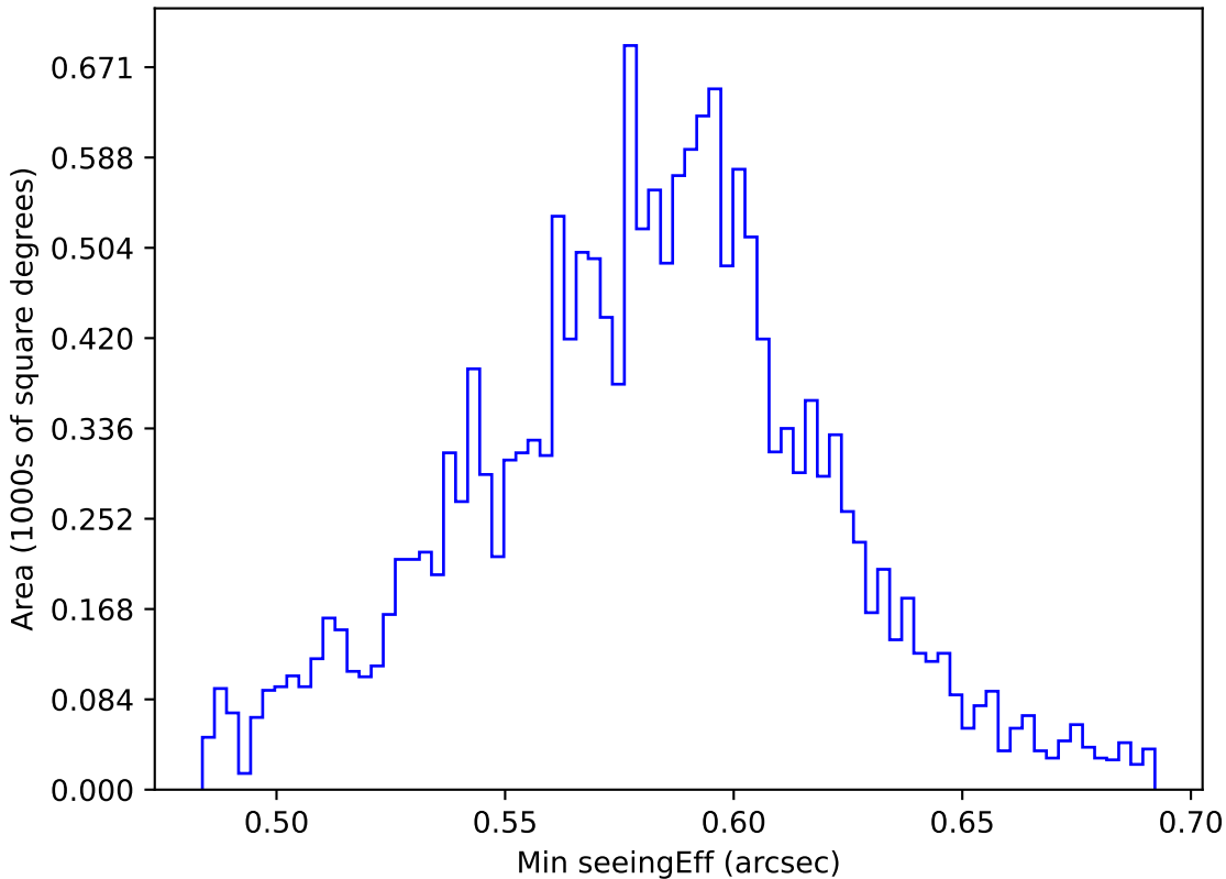
weather_cloudso20v3.4_10yrs WFD all bands: Min seeingEff
