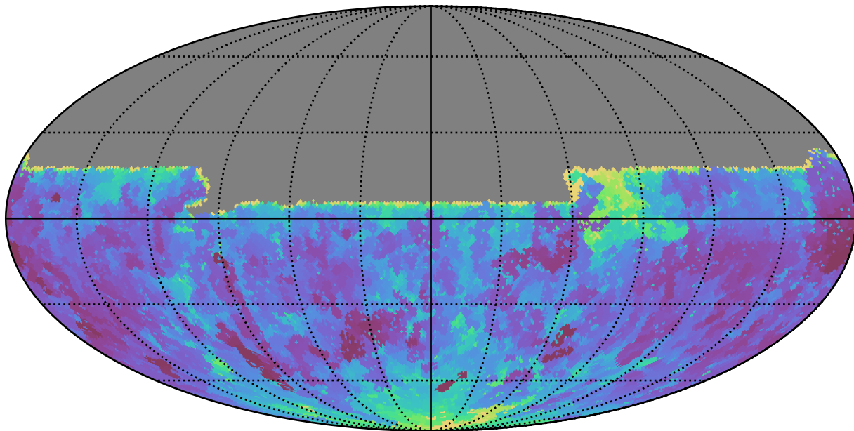
weather_cloudso20v3.4_10yrs All sky u band: Min seeingEff
