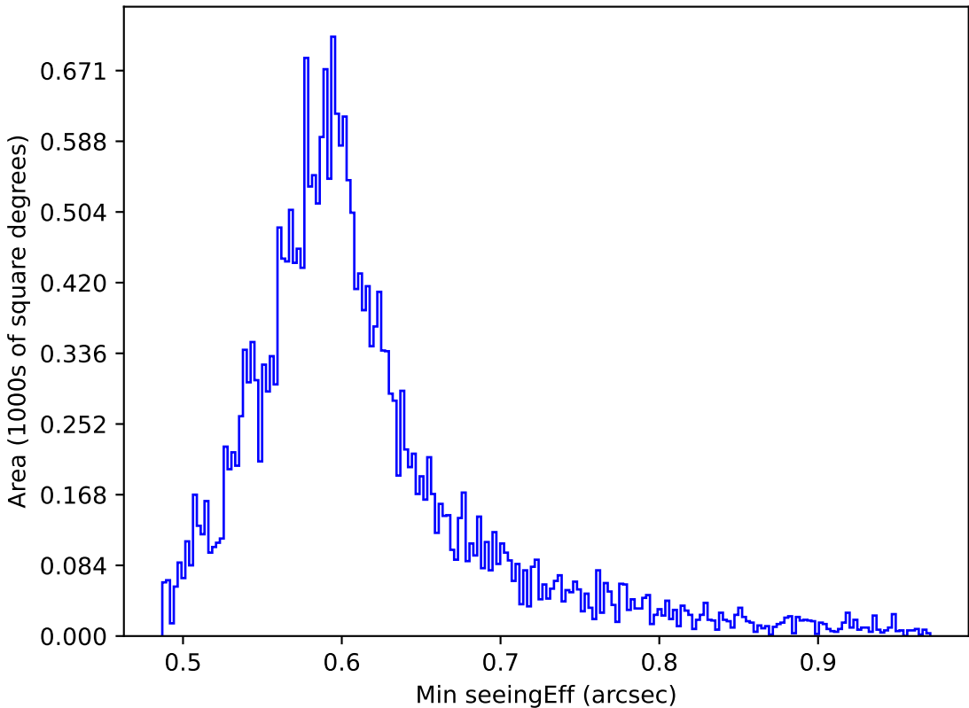
weather_cloudso20v3.4_10yrs All sky all bands: Min seeingEff
