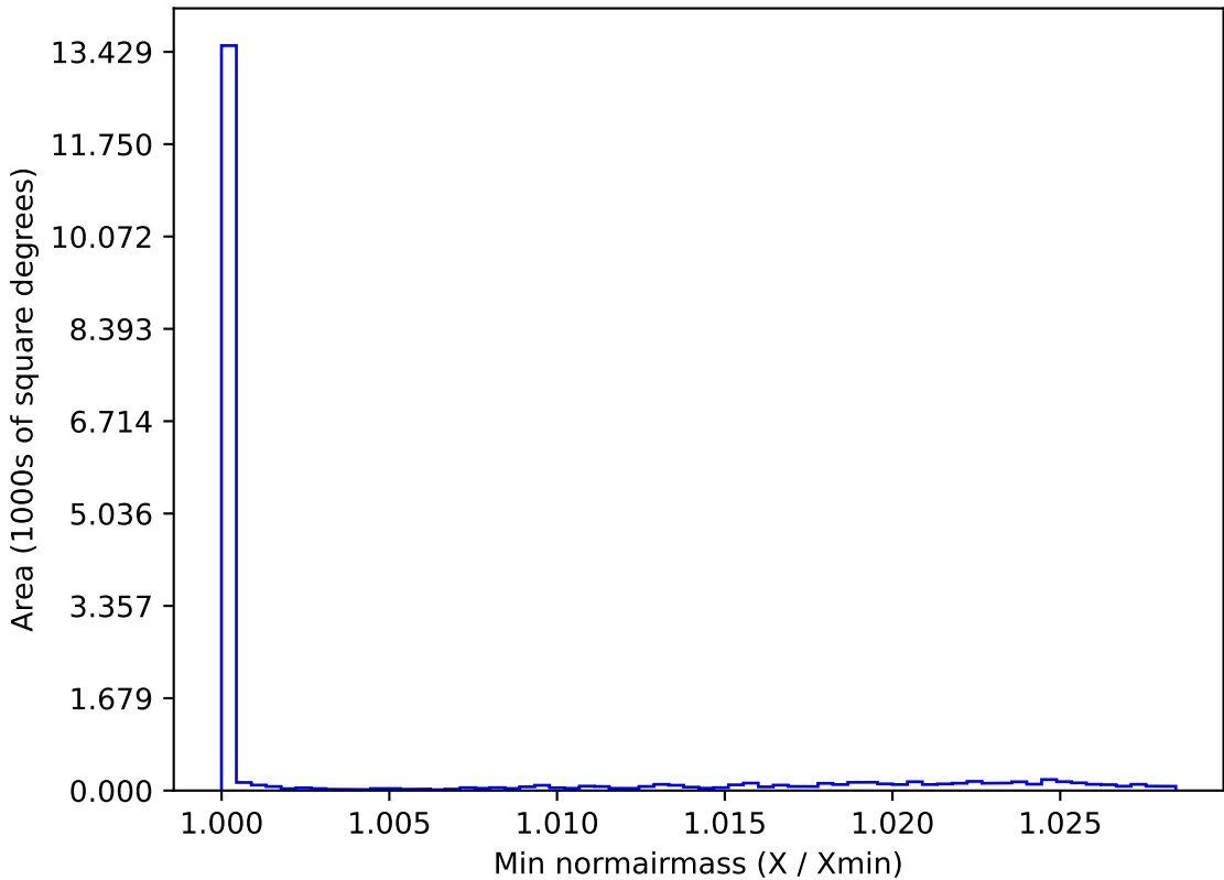
weather_cloudso20v3.4_10yrs WFD all bands: Min normairmass
