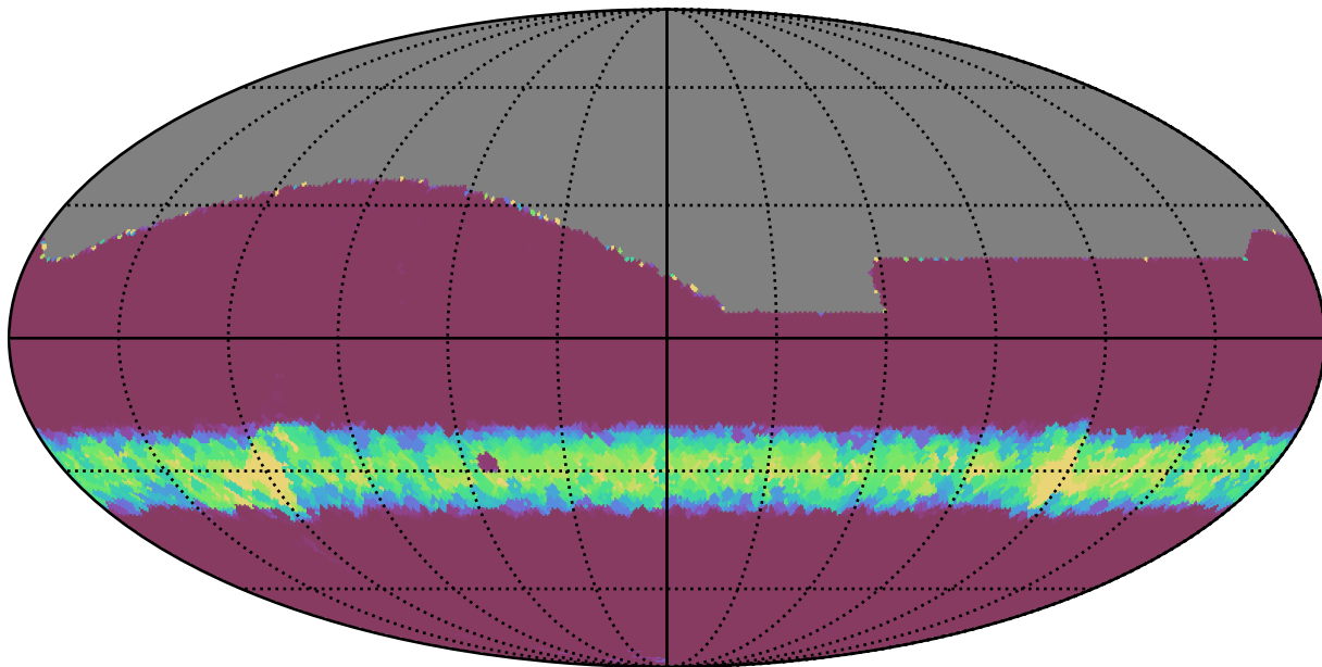
weather_cloudso20v3.4_10yrs All sky all bands: Min normairmass
