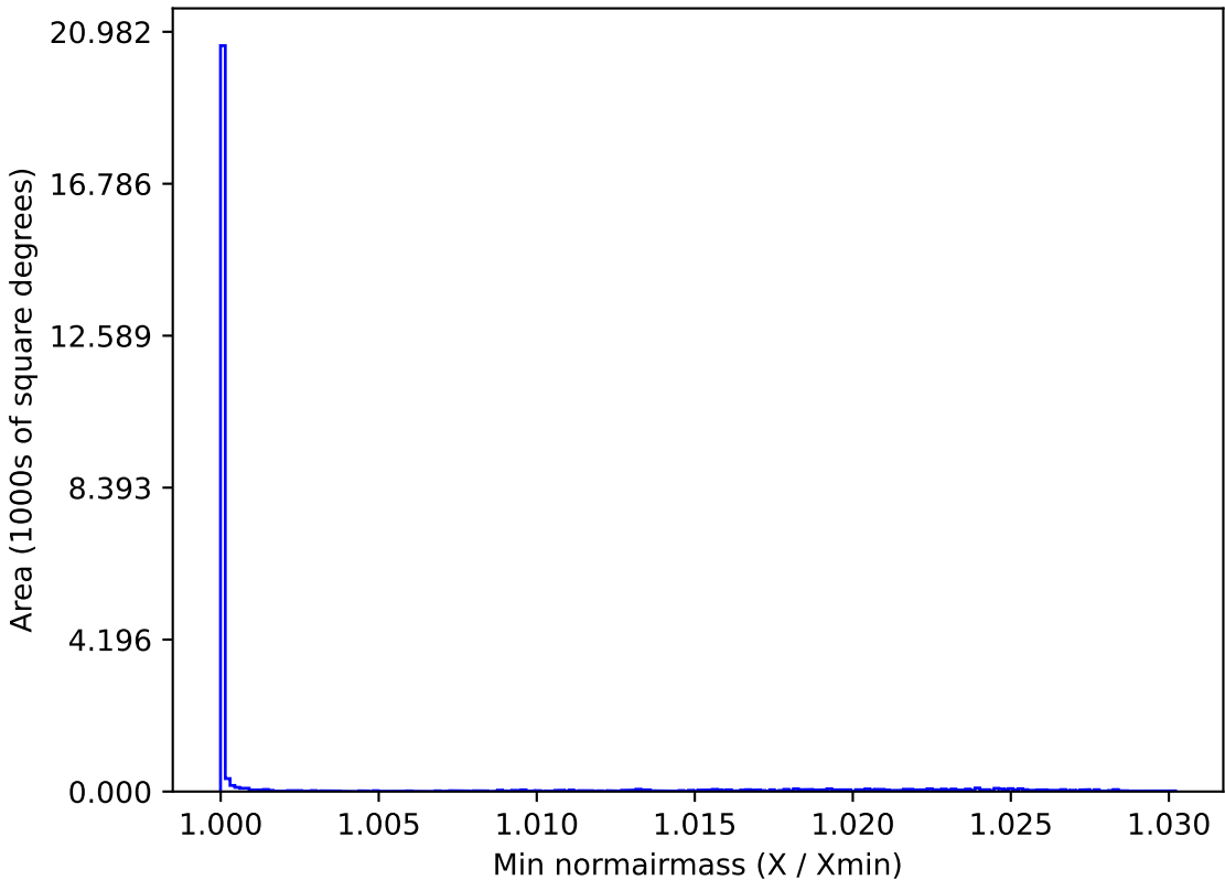
weather_cloudso20v3.4_10yrs All sky all bands: Min normairmass
