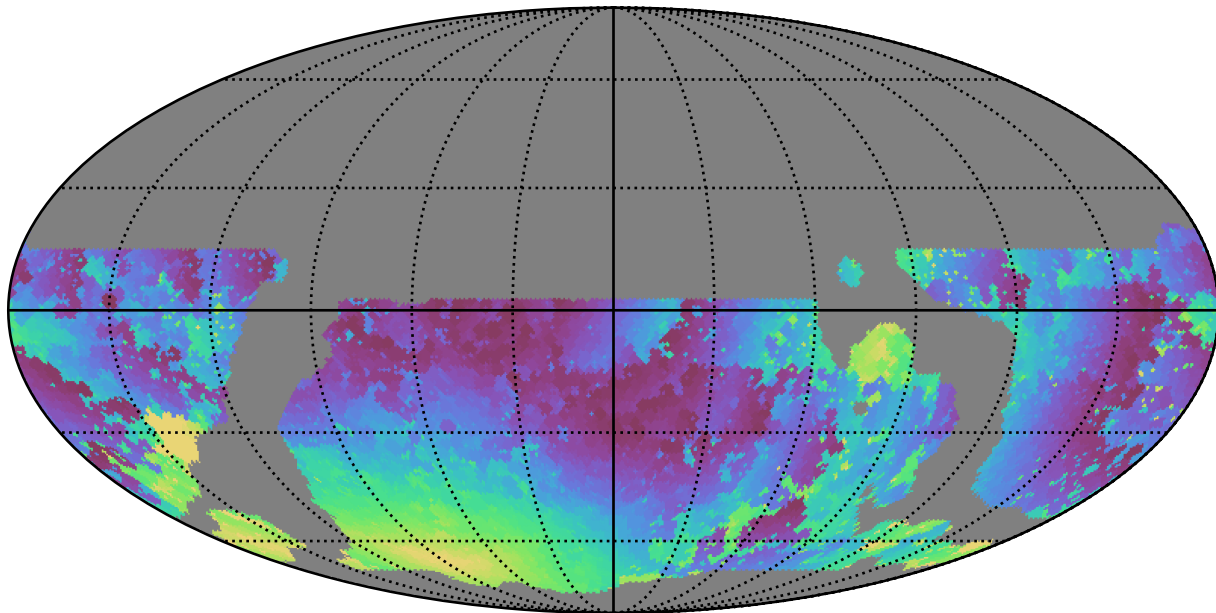
weather_cloudso20v3.4_10yrs WFD u band: Min moonDistance
