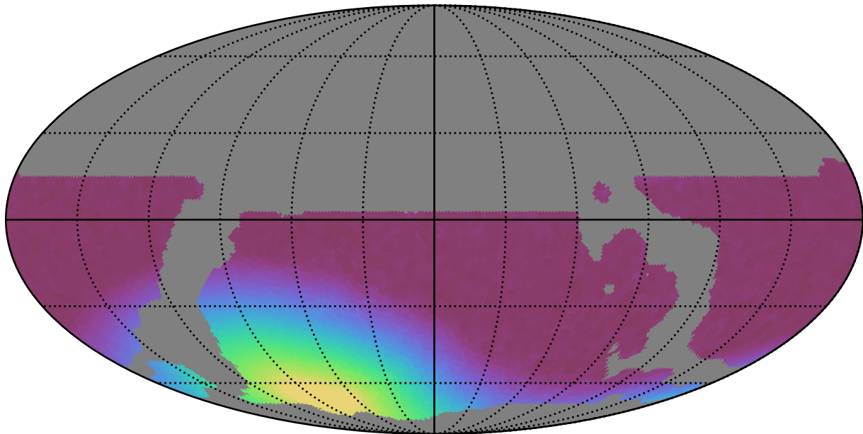
weather_cloudso20v3.4_10yrs WFD all bands: Min moonDistance
