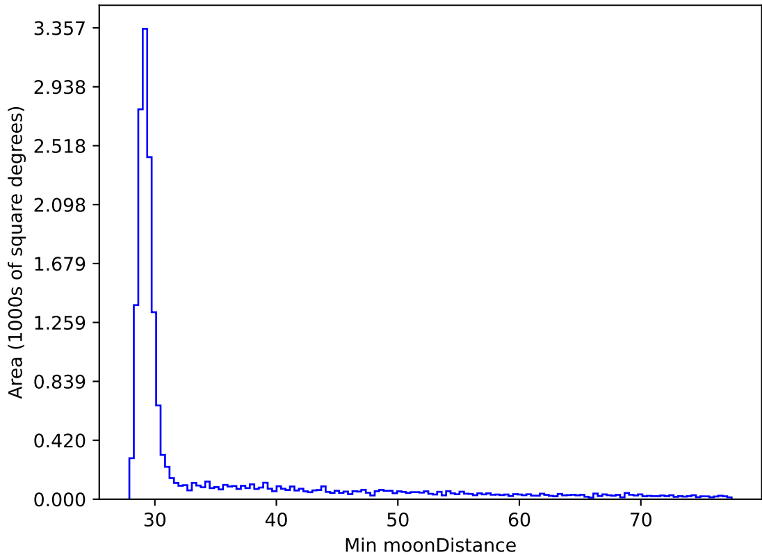
weather_cloudso20v3.4_10yrs WFD all bands: Min moonDistance
