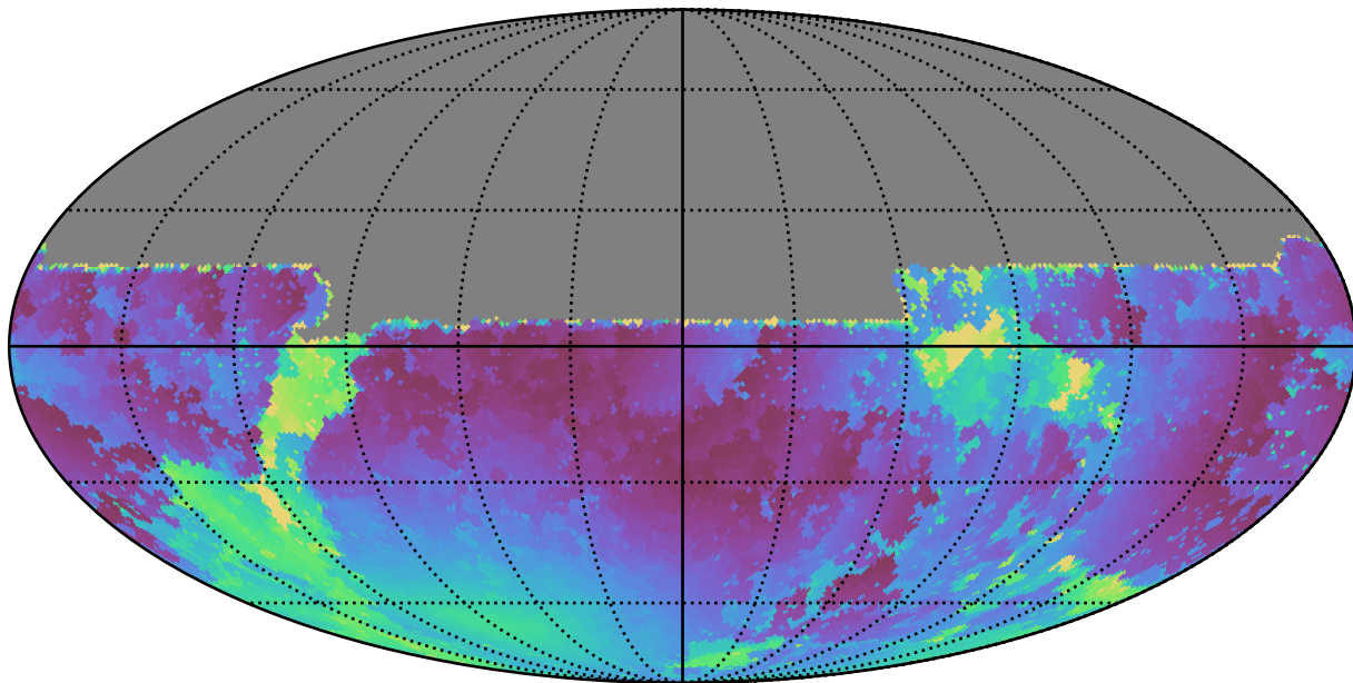
weather_cloudso20v3.4_10yrs All sky u band: Min moonDistance
