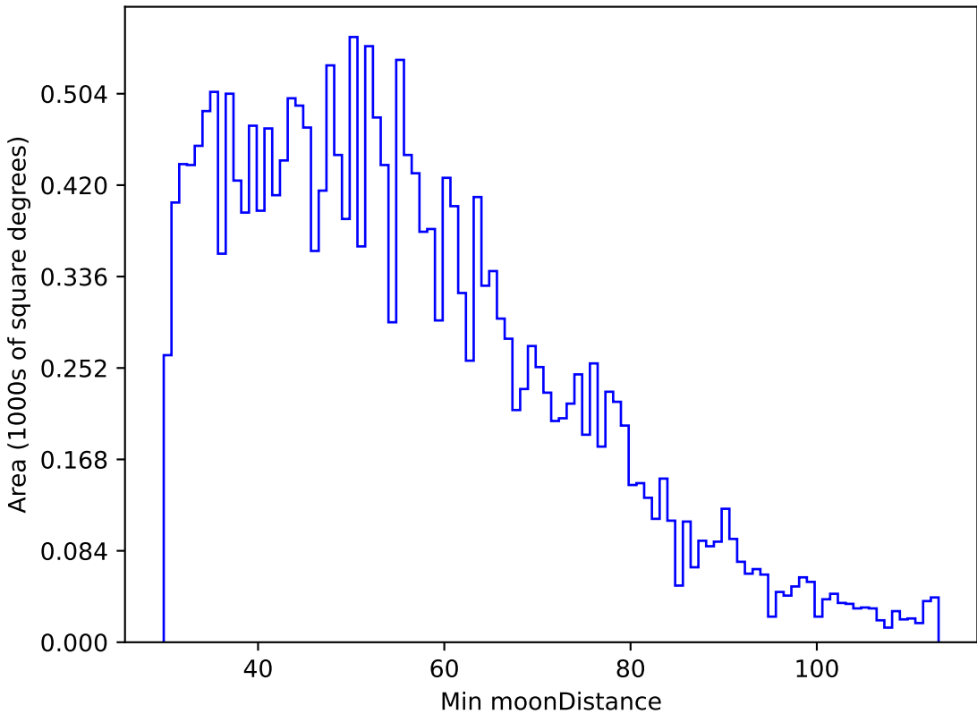
weather_cloudso20v3.4_10yrs All sky u band: Min moonDistance
